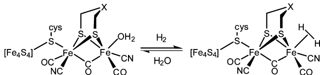
Figure 1. Relevant H 2 O/H 2 interconversion scheme with two likely intermediates in the hydrogenase-mediated reduction of protons.
