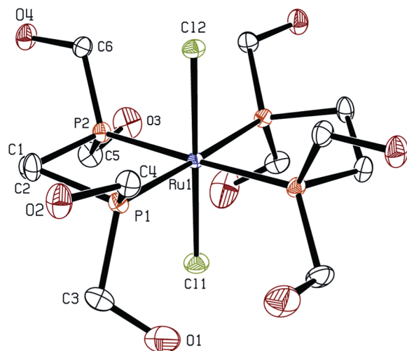
Figure 2. ORTEP representation of \text{trans-Ru}(\text{DHMPPE})_2\text{Cl}_2 ( Ib ). Ellipsoids are shown at 50% probability. Hydrogen atoms and solvent water molecules are omitted for clarity.
