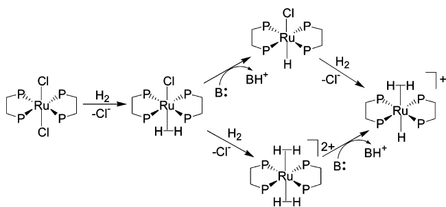
Scheme 1. Possible Pathways for the Heterolysis of H 2 a
