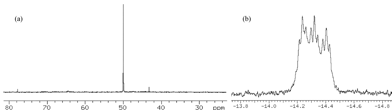
Figure 4. ^{31}\text{P}\{^1\text{H}\} NMR spectrum of (a) \text{trans-}[\text{Ru}(\text{DMeOPrPE})_2(\text{H}_2)\text{Cl}]^+ and (b) the hydride region in the ^1\text{H} NMR spectrum of the HD isotopologue, \text{trans-}[\text{Ru}(\text{DMeOPrPE})_2(\text{HD})\text{Cl}]^+ . The minor peak at \delta 44.4 in spectrum (a) is unreacted \text{trans-Ru}(\text{DMeOPrPE})_2\text{Cl}_2 .
