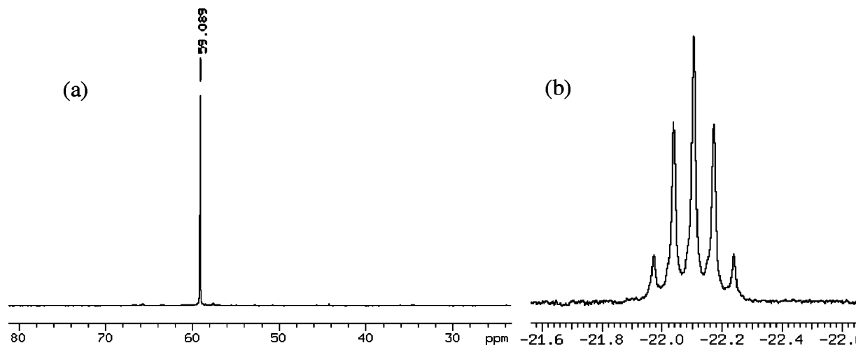
Figure 3. ^{31}\text{P}\{^1\text{H}\} NMR spectrum of (a) \text{trans-}[\text{Ru}(\text{DMeOPrPE})_2\text{HCl}] and (b) the hydride region in the ^1\text{H} NMR spectrum (b).
