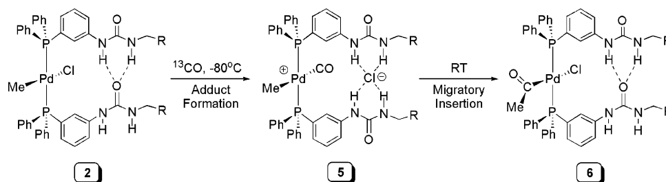
Scheme 5. Reactivity of 2 with ^{13}\text{CO}
