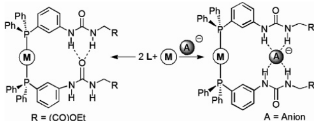
Scheme 2. Synthesis of Urea-Based Phosphine Ligand 1
