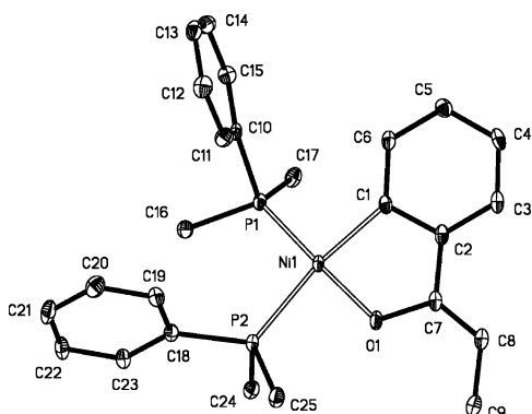
Figure 3. ORTEP perspective of compound 2d . Selected bond distances (Å) and angles (deg): Ni1–C1, 1.932(2); Ni1–O1, 1.8595(15); Ni–P1, 2.1391(6); Ni1–P2, 2.2400(7); O1–C(7), 1.347(3); C7–C8, 1.337(3); C1–Ni1–O1, 85.76(8); P1–Ni1–P2, 89.90(3).
