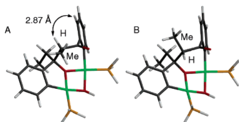
Figure 1. Molecular models of the 3b diastereomeric pair (PMe 3 ligands have been replaced by PH 3 ): (A) major isomer ( R,R or S,S ), showing the C(En)H...H( ortho ) approach; (B) minor isomer ( R,S or S,R ).
