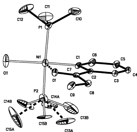
Figure 2. ORTEP view of 1b . Selected bond lengths (Å) and angles (deg): Ni1–C1, 1.885(3); Ni1–P1, 2.1907(10); Ni1–P2, 2.1775(10); Ni1–Cl1, 2.2375(11); Ni1–O1, 2.472(2); C7–O1, 1.222(4); C1–Ni1–O1, 77.60(11); Ni1–C1–C2, 118.5(2); P1–Ni1–P2, 169.15(4).
