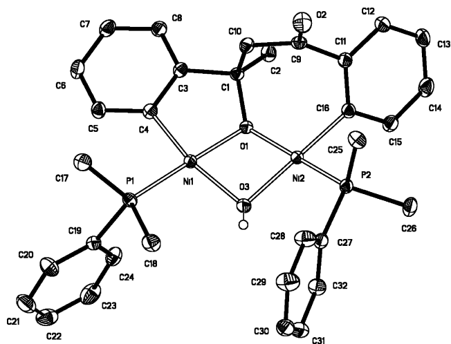
Figure 4. ORTEP perspective of compound 3c . Selected bond distances (Å) and angles (deg): Ni1–O1, 1.8945(10); Ni1–O3, 1.8986(11); Ni2–O1, 1.9060(10); Ni1–P1, 2.1436(4); Ni2–P2, 2.1221(4); Ni1–C4, 1.8790(14); Ni2–C16, 1.8839(14); C9–O2, 1.2227(18); C1–O1, 1.4665(16); Ni1···Ni2, 2.8312(3); Ni1–O1–Ni2, 96.31(4); Ni–O3–Ni2, 96.08(5); Ni1–O1–Ni2–O3, 21.15(5).
