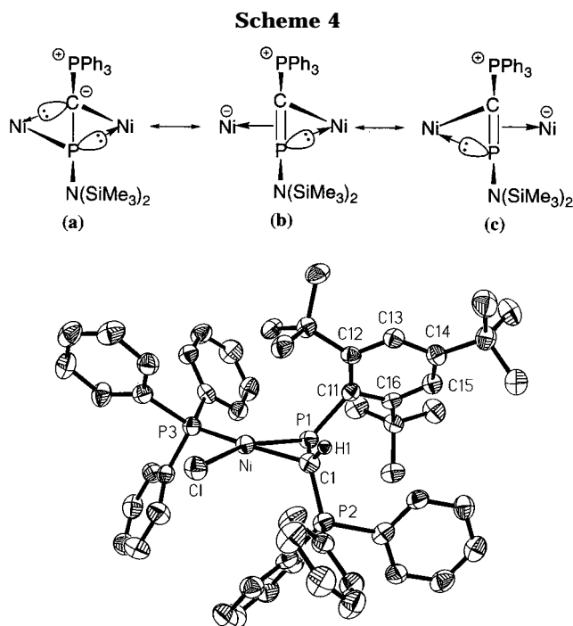
Figure 2. Thermal ellipsoid drawing of Cl(PPh 3 )Ni[η 2 -C(H)(PPh 3 )=P(Mes*)] ( Va ).
