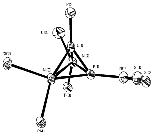
Figure 1. Thermal ellipsoid drawing of \text{Ni}_2\text{Cl}_2(\text{PPh}_3)_2[\mu_2\text{-}\eta^2\text{-}\eta^2\text{-C}(\text{PPh}_3)=\text{PN}(\text{SiMe}_3)_2] ( IIIa ) with the phenyl and methyl groups removed for clarity.
