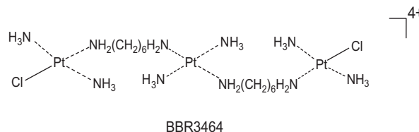
Figure 1. Structure of BBR3464.
