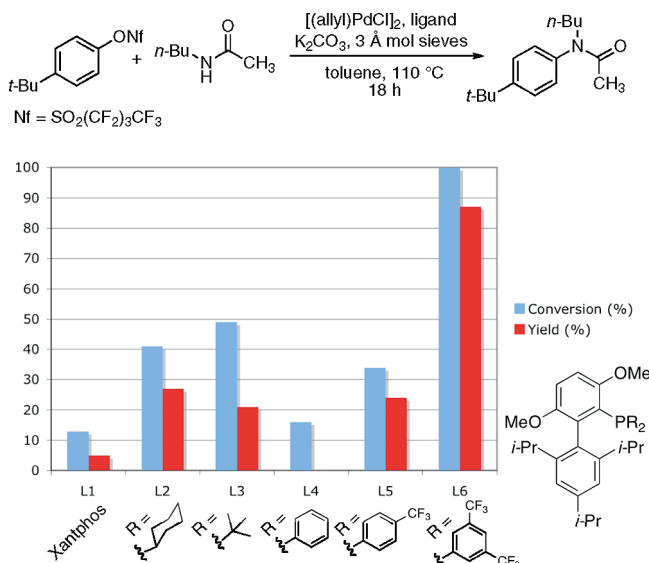
Chart 1. Ligand Optimization for the Coupling of 4- tert -Butylphenyl Nonaflate and N -Butyl Acetamide a
