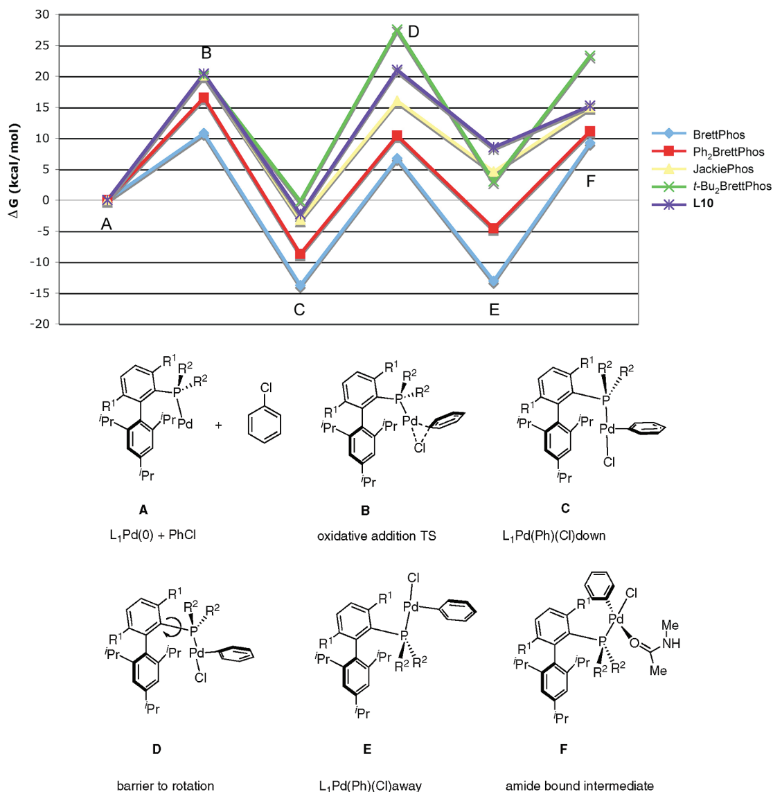
Figure 5. Partial potential energy diagram of the catalytic cycle with biarylmonophosphine-Pd catalysts.
