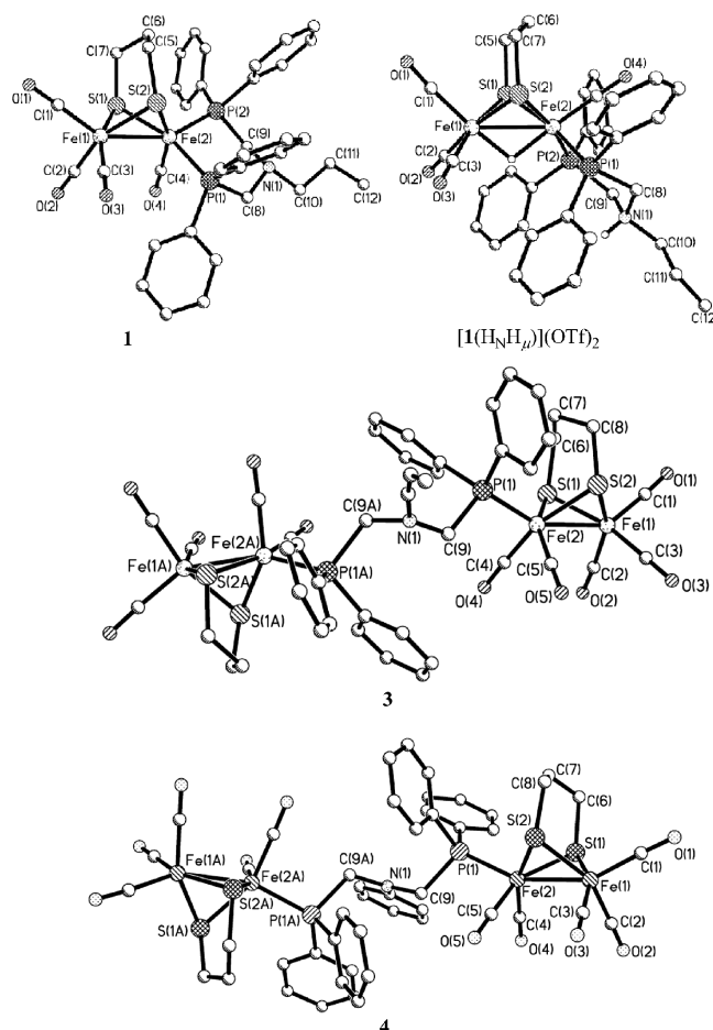
Figure 1. Molecular structures of 1 , 3 , 4 , and [\text{I}(\text{H}_\text{N}\text{H}_\mu)](\text{OTf})_2 as ball and stick drawings.
