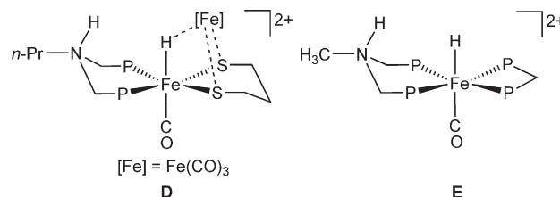
Figure 6. Comparison of the Structures of [(\mu-H)Fe(\mu-pdt)(CO)\{Ph_2PCH_2N(n-Pr)CH_2PPh_2\}]^{2+} unit ( D ) in [1(H_NH_\mu)]^{2+} and the DuBois' complex trans-[HFe(dmpm)(CO)\{Et_2PCH_2N(CH_3)CH_2PEt_2\}]^{2+} ( E ).
