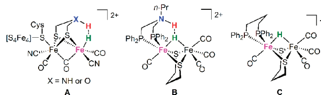
Figure 5. Structures of the proposed [\text{2Fe2S}] subcluster with a t -hydride ( A , t = terminal), the \mu -hydride diiron mimic [\mathbf{1}(\text{H}_\text{N}\text{H}_\mu)]^{2+} ( B ), and the \mu -hydride complex [\mathbf{5}(\text{H}_\mu)]^+ ( C ).
