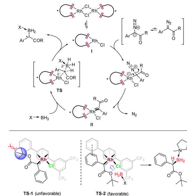
Scheme 1. Proposed B–H Insertion Mechanism
