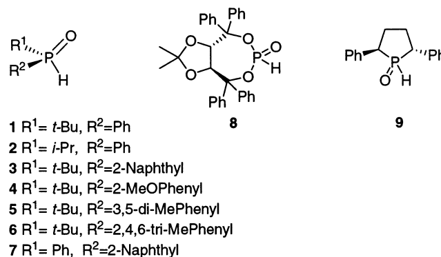
Figure 1. Secondary phosphine oxides.
