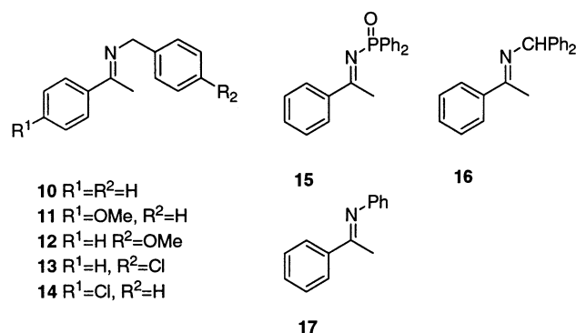
Figure 2. Imines.
