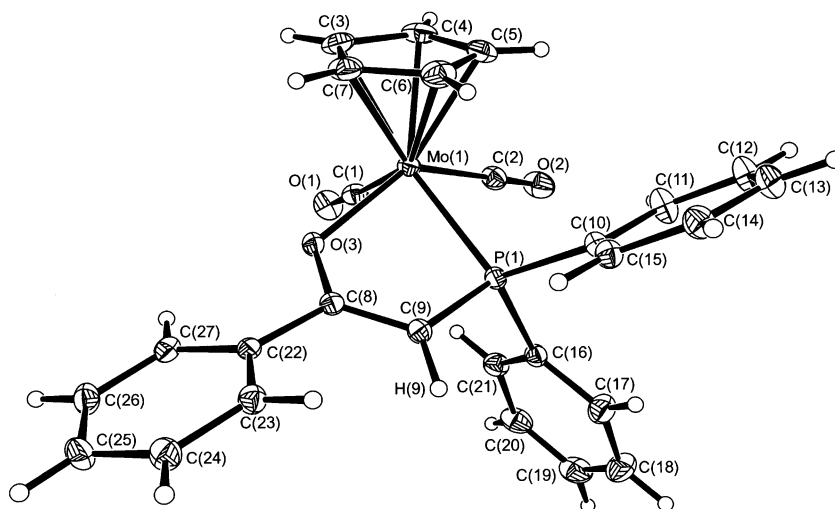
Fig. 2. Molecular structure of [\text{Mo}(\text{CO})_2\{\text{PPh}_2\text{CH}=\text{C}(\text{O})\text{Ph}-\kappa^2\text{P},\text{O}\}(\eta^5\text{-C}_5\text{H}_5)] ( 9 ) with thermal ellipsoids shown at the 30% probability level.
