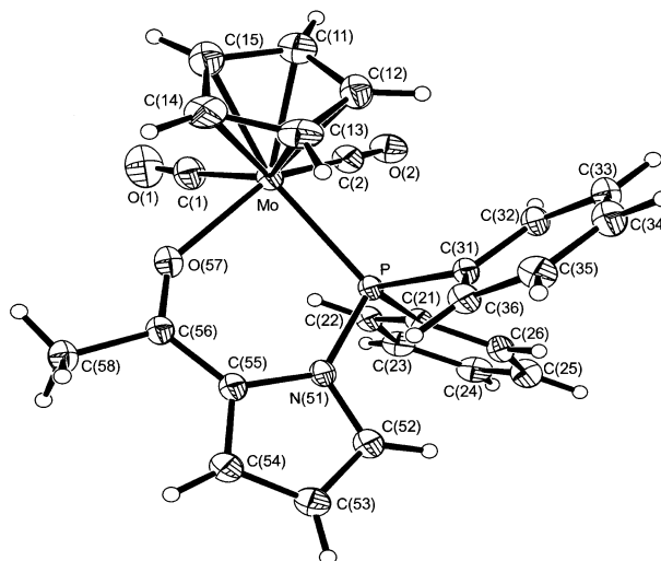
Fig. 1. Structure of the cation present in [\text{Mo}(\text{CO})_2(\text{L}^1\text{-}\kappa^2P,O)(\eta^5\text{-C}_5\text{H}_5)]\text{BF}_4 ( 4a ) with thermal ellipsoids shown at the 30% probability level.
