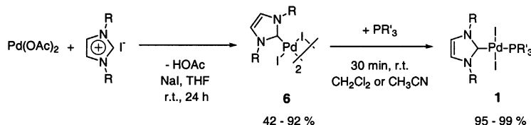
Scheme 2. Preparation of complexes 1a–1l and 6a–6c .
