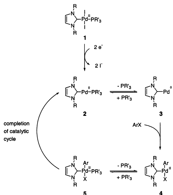
Scheme 1. Proposed mechanism for the oxidative addition of aryl halides to mixed NHC/phosphine complexes of palladium.
