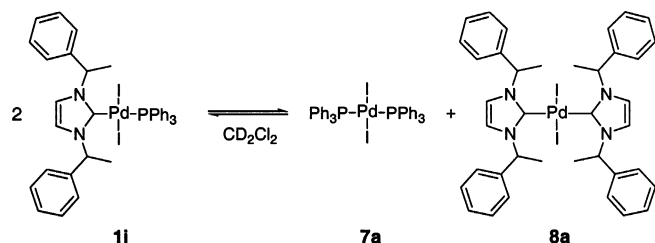
Scheme 3. Ligand exchange. Equilibrium of the complexes 1i , 7a and 8a .
