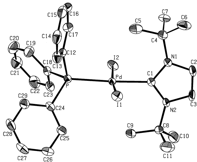
Fig. 1. Molecular structure of trans -diiodo(1,3-di- tert -butylimidazolin-2-ylidene)(triphenylphosphino)palladium(II) ( 1e ). Thermal ellipsoids are drawn at the 50% probability level. For clarity the hydrogen atoms are omitted and only one part of the distorted atoms is shown. Selected bond lengths (Å) and angles (°): Pd–P = 2.334(1), Pd–C1 = 2.031(4), Pd–I1 = 2.6325(8), Pd–I2 = 2.6175(8), P–Pd–C1 = 175.5(1), I1–Pd–I2 = 173.33(2), N1–C1–N2, 105.7(3), Pd–P–C12 = 105.5(1), Pd–P–C18 = 119.8(1), Pd–P–C24 = 118.9(1).
