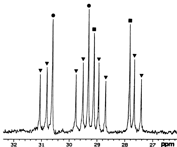
Fig. 2. ^{31}\text{P}\{^1\text{H}\} -NMR spectrum (121.4 MHz, 20^\circ\text{C} ) of the solution resulting from the addition of one equivalent of [\text{Rh}(\text{NBD})\{\text{P}(p\text{-Tol})_3\}_2]\text{BF}_4 to a chloroform- d_1 solution of [\text{Rh}(\text{NBD})(\text{PPh}_3)_2]\text{BF}_4 (■ [\text{Rh}(\text{NBD})(\text{PPh}_3)_2]\text{BF}_4 ; ● [\text{Rh}(\text{NBD})\{\text{P}(p\text{-Tol})_3\}_2]\text{BF}_4 ; ▼ [\text{Rh}(\text{NBD})(\text{PPh}_3)\{\text{P}(p\text{-Tol})_3\}]\text{BF}_4 ).
