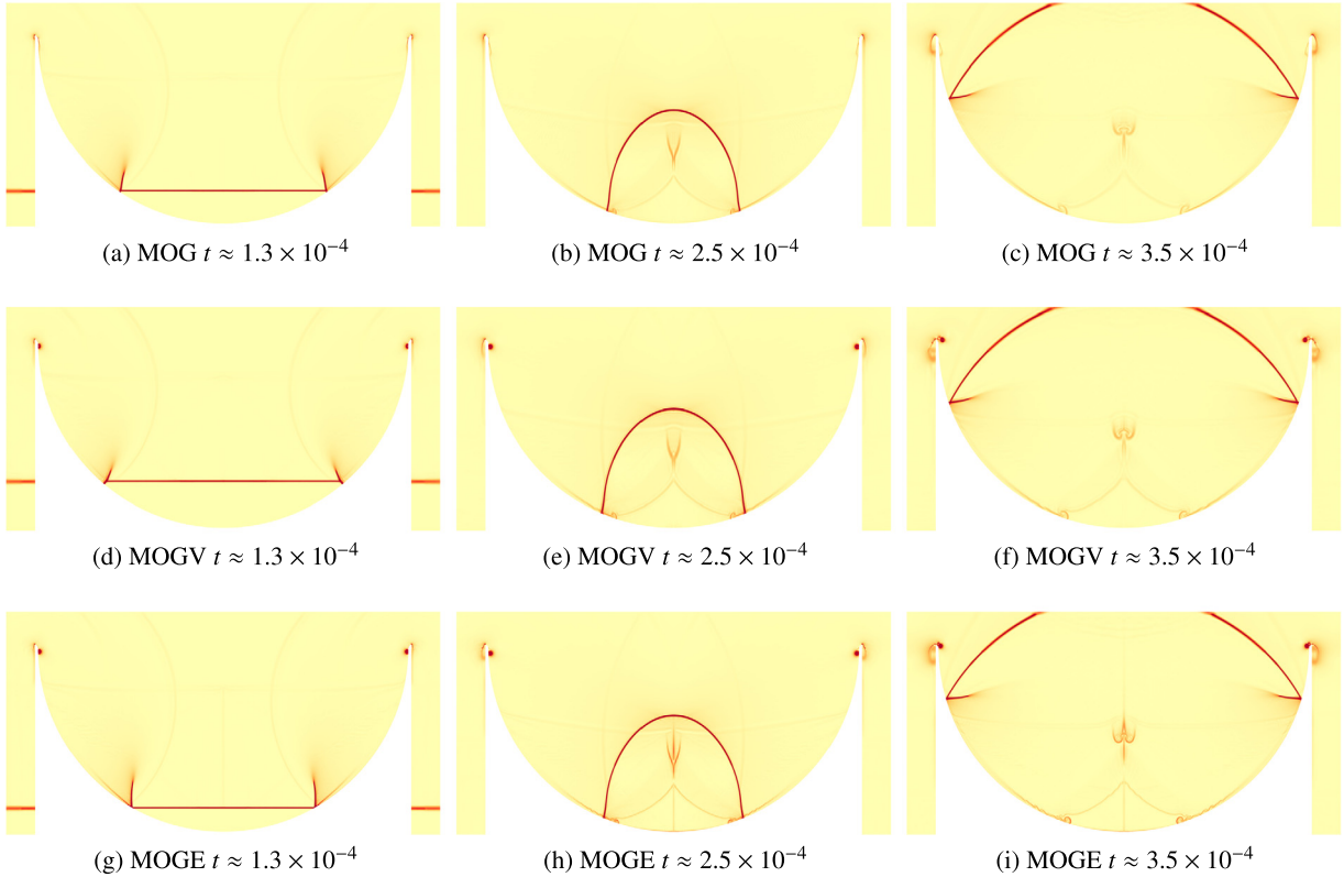
Fig. 22. Distribution of the density gradient magnitude with 4th-order limiters for the shock on cylindrical cavity test problem at different times. The MOGE scheme provides the sharpest resolution of all the flow features, compared to the other two schemes.
