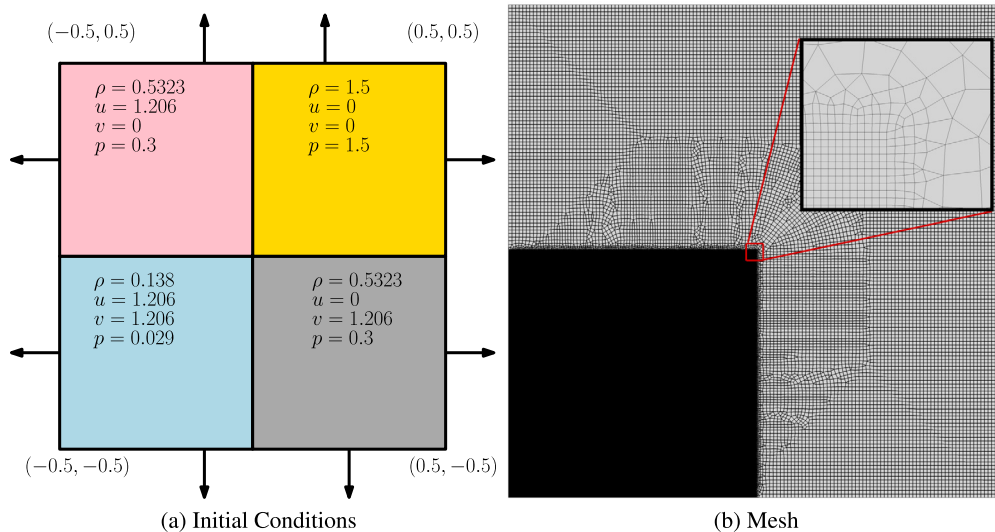
Fig. 19. Initial conditions and mesh for the multidimensional Riemann problem.
