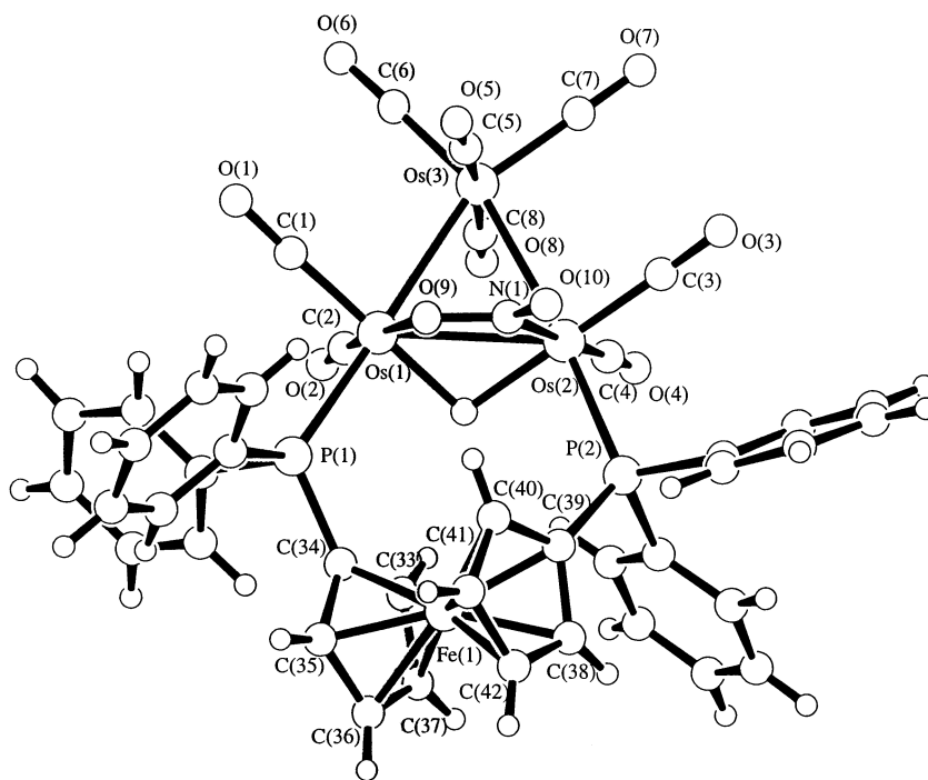
Fig. 1. The molecular structure of [\text{Os}_3(\mu\text{-H})(\text{CO})_8(\mu\text{-}\eta^2\text{-NO}_2)(\mu\text{-dppf})] ( 2 ) with the atom-numbering scheme.
