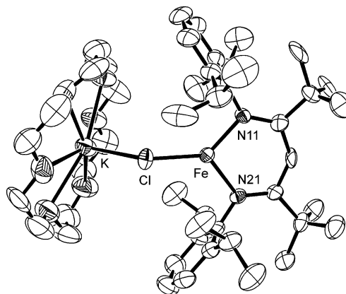
Figure 9. X-ray crystal structure of L^{\text{tBu}}\text{FeClK}(18\text{-crown-6}) . Thermal ellipsoids shown at 50% probability. Hydrogen atoms, minor conformer of tert -butyl group, and toluene solvate omitted for clarity. Selected bond lengths (Å) and angles ( ^\circ ): Fe–N11 1.934(6), Fe–Cl 2.235(3), K–O 2.850(9), 2.741(7), 2.952(9), 2.848(10), 2.830(9), 2.774(8), K–Cl 3.074(3); N11–Fe–N21 101.8(3), N11–Fe–Cl 134.3(2), N21–Fe–Cl 123.8(2), Fe–Cl–K 134.17(11).
