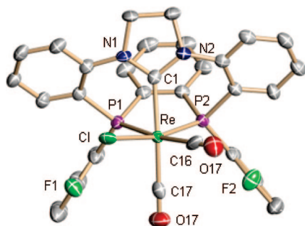
Figure 6. Molecular structure of complex [11] in [11]·0.25H 2 O·CH 2 Cl 2 . Selected bond lengths (Å) and bond angles (deg): Re–P1 2.3732(11), Re–P2 2.2866(11), Re–Cl1 2.5234(12), Re–Cl2 2.156(4), Re–C16 1.997(6), Re–C17 1.961(5); P1–Re–P2 82.96(4), P1–Re–Cl1 95.68(4), P1–Re–Cl2 79.31(11), P1–Re–C16 172.68(14), P1–Re–C17 93.81(14), P2–Re–Cl1 166.53(4), P2–Re–Cl2 80.63(11), P2–Re–C16 91.99(13), P2–Re–C17 95.34(12), Cl1–Re–Cl2 85.94(11), Cl1–Re–C16 88.00(13), Cl1–Re–C17 98.13(12), C1–Re–C16 94.7(2), C1–Re–C17 172.4(2), C16–Re–C17 91.9(2), N1–C1–N2 107.0(4).
