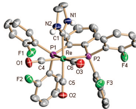
Figure 3. Molecular structure of the complex cation [H_2-6]^+ in [H_2-6]Cl \cdot 3THF . Selected bond lengths (Å) and angles (deg): Re–P1 2.428(2), Re–P2 2.420(2), Re–C1 2.188(5), Re–C4 1.971(5), Re–C5 1.950(5), Re–C6 1.975(6); P1–Re–P2 80.11(5), P1–Re–C1 90.60(13), P1–Re–C4 93.54(14), P1–Re–C5 90.50(15), P1–Re–C6 173.31(14), P2–Re–C1 90.43(13), P2–Re–C4 173.60(14), P2–Re–C5 91.53(15), P2–Re–C6 93.21(15).
