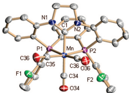
Figure 8. Molecular structures of [14]^+ in [14]\text{Br}\cdot\text{CH}_2\text{Cl}_2 . Selected bond lengths (Å) and angles (deg): Mn–P1 2.2469(7), Mn–P2 2.2386(8), Mn–C1 2.033(2), Mn–C34 1.813(2), Mn–C35 1.823(2), Mn–C36 1.828(3), N1–C1 1.355(3), N2–C1 1.345(3); P1–Mn–P2 84.64(2), P1–Mn–C1 81.67(7), P1–Mn–C34 92.56(8), P1–Mn–C35 92.21(8), P1–Mn–C36 173.82(8), P2–Mn–C1 81.60(7), P2–Mn–C34 93.31(8), P2–Mn–C35 172.59(8), P2–Mn–C36 91.85(8), C1–Mn–C34 172.60(9), C1–Mn–C35 91.32(10), C1–Mn–C36 92.79(10), C34–Mn–C35 93.54(11), C34–Mn–C36 92.73(11), C35–Mn–C36 90.66(11), N1–C1–N2 107.2(2).
