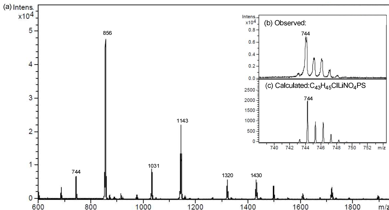
Figure 2. Complex formation between 21a and Cy-DHTP (0.4 equiv.) in the presence of t -BuOLi (1.4 equiv.) as observed by ESI-TOF-MS in the negative ion mode. (a) ESI-TOF mass spectrum obtained following stirring for 30 min. Detailed view of (b) the observed isotopic distribution compared to (c) the theoretical isotopic pattern of the complex shown in Figure 3.
