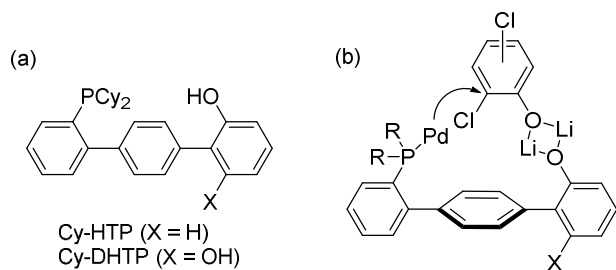
Figure 1. (a) Hydroxyterphenylphosphines and (b) assumed heteroaggregates.
