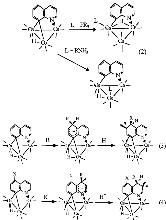
Figure 1. \mu_3\text{-}\eta^2 electron-deficient benzoheterocycle triosmium complexes.
