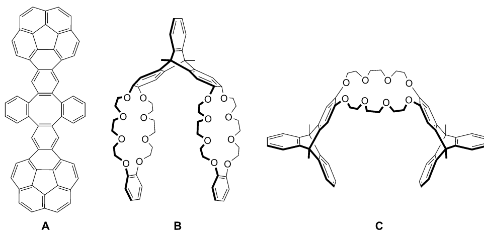
Fig. 1. Structures of some molecular tweezers
