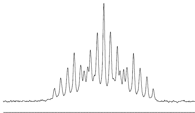
Fig. 2. ^{31}\text{P}\{^1\text{H}\} NMR spectrum of \text{Ph}_2\text{PC(O)(CF}_2)_6\text{CF}_3 , (4).
