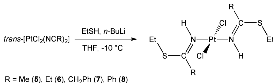
Scheme 3. Synthesis of the Imino Thioether Complexes \text{trans-[PtCl}_2\{\text{E-N(H)=C(SET)R}\}_2]
