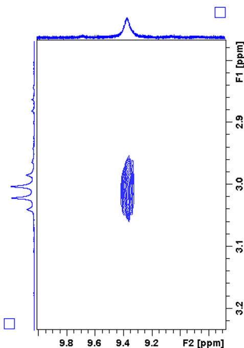
Figure 1. Portion of 400 MHz NOESY Spectrum of 7 showing the correlation peak between Pt–NH and -\text{SCH}_2- protons.
