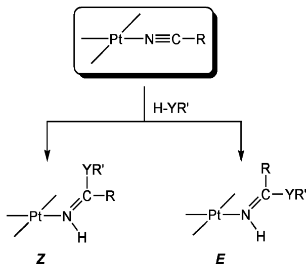
Scheme 1. Configuration of Iminoether and Amidine Complexes
