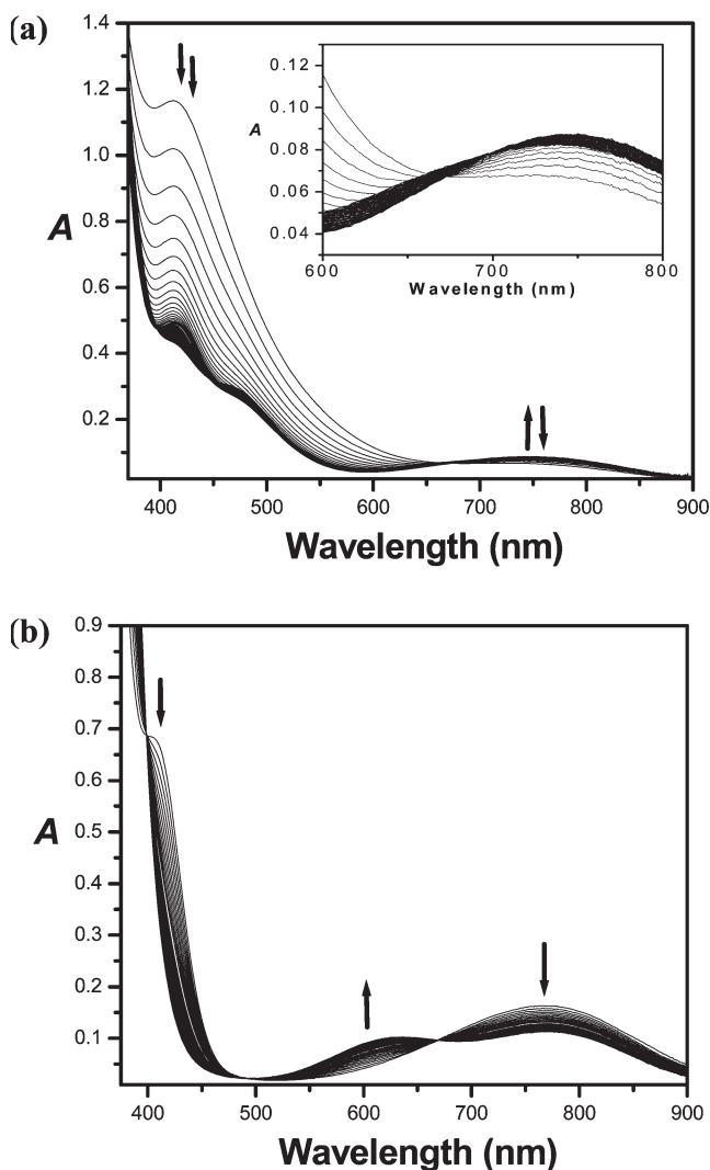
Figure 3. UV-visible spectral changes in MeCN. (a) During the oxidation of \text{PMe}_3 by 1a at 10 °C, [\mathbf{1a}]:[\text{PMe}_3] = 1:20 ( [\mathbf{1a}] = 0.35 \text{ mM} ); time interval between each scan = 1.4 min. The inset shows the absence of an isosbestic point. (b) Decomposition of 2a at 22 °C, [\mathbf{2a}] = 2.53 \text{ mM} , time interval between each scan = 5.5 min.
