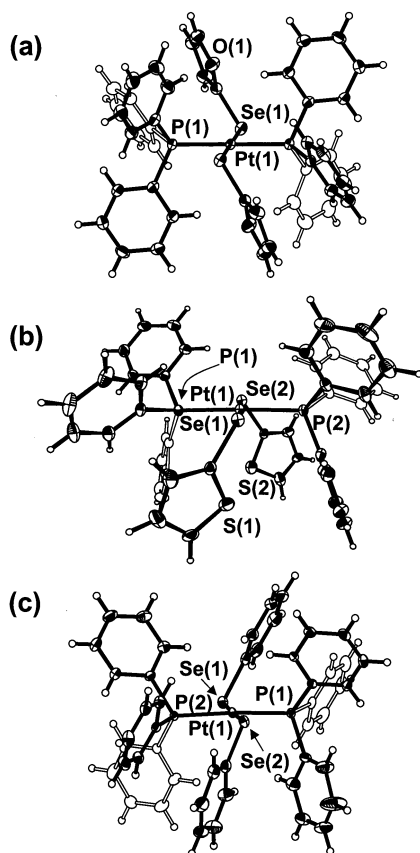
Fig. 2. The molecular structures of (a) trans-anti -[Pt(SeFu) 2 (PPh 3 ) 2 ] ( 1ta ), (b) trans-syn -[Pt(SeTh) 2 (PPh 3 ) 2 ] [ 10 ], and (c) trans-anti -[Pt(SePh) 2 (PPh 3 ) 2 ] [ 17 ] indicating the numbering of the atoms. The thermal ellipsoids have been drawn at 50% probability level.
