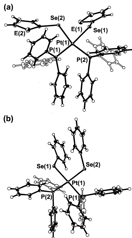
Fig. 1. The molecular structures of (a) cs -[Pt(SeFu) 2 (PPh 3 ) 2 ] ( 1cs ) and ca -[Pt(SeTh) 2 (PPh 3 ) 2 ] ( 2ca ), and (b) ca -[Pt(SePh) 2 (PPh 3 ) 2 ] ( 3ca ) (adapted from data in Ref. [17]) indicating the numbering of the atoms. The thermal ellipsoids have been drawn at 50% probability level.
