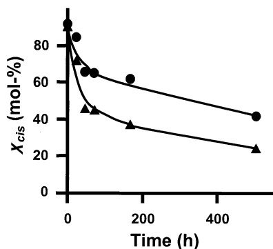
Fig. 5. Isomerization of cis -[Pt(SeTh) _2 (PPh _3 ) _2 ] in \text{CH}_2\text{Cl}_2 (●) and \text{C}_6\text{H}_6 (▲). The relative content of the cis -isomer \chi_{cis} (mol.%) has been determined from the relative intensities of the ^{31}\text{P} resonances of cis - and trans -[Pt(SeTh) _2 (PPh _3 ) _2 ].
