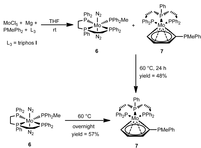
Scheme 3. One-Pot Synthesis of \text{Mo}^0 Complexes 6 and 7 with a Tridentate Phosphine Ligand
