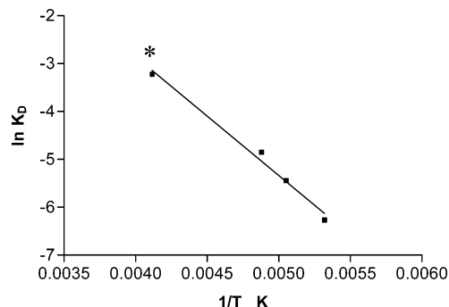
Figure 4. Plot of \ln K_D as a function of 1/T for the dissociation of \text{Pd}[\text{PCy}_3]_3 ( R^2 = 0.988 ) (* point from ref 2g).
