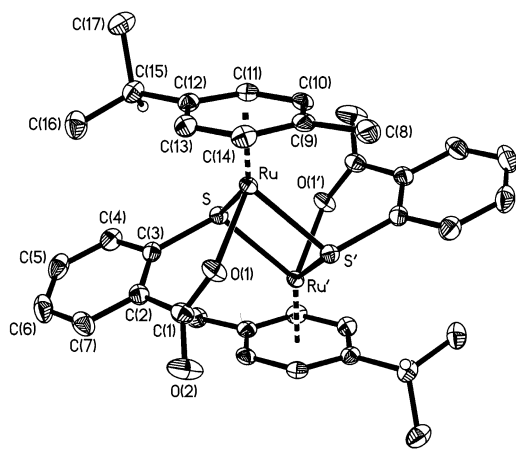
Fig. 3. Molecular structure of [(p\text{-cymene})\text{Ru}(\text{tsal})]_2 ( 3 ) showing the atom numbering scheme. Thermal displacement ellipsoids are shown at 50% probability, and all hydrogen atoms [except the isopropyl hydrogens H(15a) and H(15a')] have been omitted for clarity.
