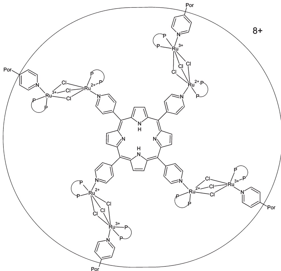
Scheme 3. Suggested Structure of the \{\text{TPyP}[\text{Ru}(\text{dppb})]_4(\mu\text{Cl}_3)_2\}_{4n2+} Film Formed on the ITO Electrode Surface
