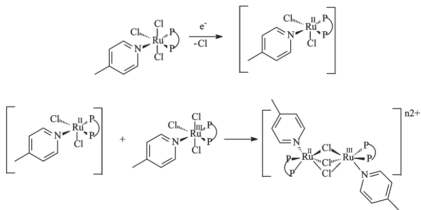
Scheme 2. Suggested Mechanism of the Formation of the \{\text{TPyP}[\text{Ru}(\text{dppb})]_4(\mu\text{Cl}_3)_2\}_{2n}^{4n2+} Film on the ITO Electrode Surface
