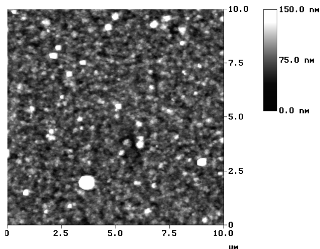
Figure 8. AFM image of a \{\text{CoTPyP}[\text{Ru}(\text{dppb})]_4(\mu\text{Cl}_3)_2\}_{4n2+} film deposited on an ITO electrode surface.
