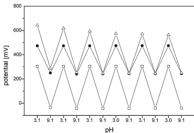
Figure 9. Stability of electrodes modified with \{\text{TPyP}[\text{Ru}(\text{dppb})_4(\mu\text{Cl}_3)_2]_{2n}\}^{4n2+} (270 cycles): crude Pt ( \Delta ), modified Pt ( \bullet ), and glass ( \square ) electrodes.
