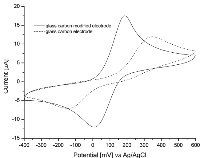
Figure 11. Cyclic voltammogram of a glass carbon electrode modified with \{\text{CoTPyP}[\text{Ru}(\text{dppb})_4(\mu\text{Cl}_3)_2]_{2n}\}^{4n2+} using catechol as a test analyte (NaTFA 0.1 \text{ mol L}^{-1} , pH = 4.5, sweep rate = 50 \text{ mV/s} ).
