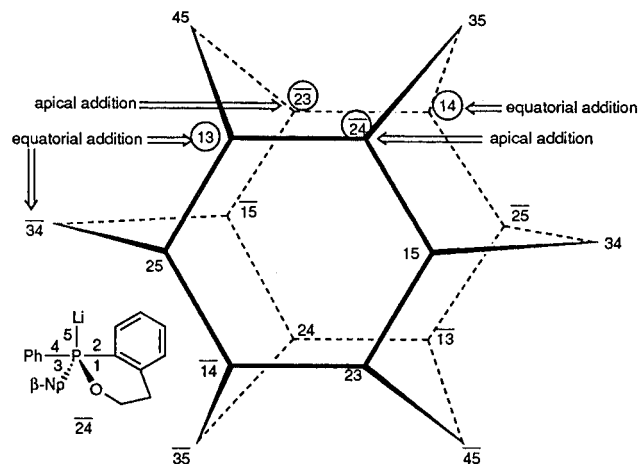
Figure 1. Desargues–Levi diagram.
