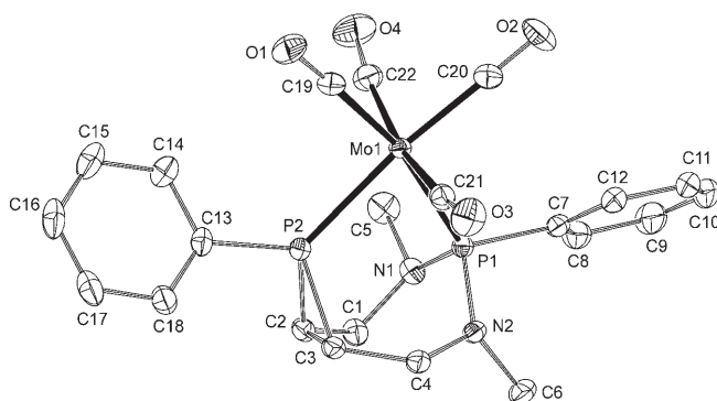
Figure 1. Structure of 19 (displacement ellipsoid plot drawn at the 50% probability level). Hydrogen atoms have been omitted for clarity. Selected bond lengths [Å], angles, and torsion angles [°]: Mo1–P1 2.5079(4), Mo1–P2 2.4917(4), P1–N1 1.7144(13), P1–N2 1.6726(13), P2–C2 1.8538(15), P2–C3 1.8317(16), C1–N1 1.474(2), C4–N2 1.4760(19), C5–N1 1.470(2), C6–N2 1.4701(19), C1–C2 1.535(2), C2–C3 1.526(2), C3–C4 1.525(2); P1–Mo1–P2 76.240(13), P1–Mo1–C20 98.26(5), P1–Mo1–C21 92.30(4), P1–Mo1–C22 95.44(5), P2–Mo1–C19 91.82(5), P2–Mo1–C21 92.12(5), P2–Mo1–C22 99.07(5), Mo1–P1–N1 115.26(5), Mo1–P1–N2 114.10(5), Mo1–P1–C7 118.07(5), Mo1–P2–C13 125.31(5), N1–P1–N2 101.81(7), C2–P2–C3 48.90(7), P1–N1–C1 114.99(10), P1–N2–C4 121.49(10), P1–N1–C5 117.16(11), P1–N2–C6 121.21(11), P2–C2–C3 64.79(8), P2–C3–C2 66.30(8), P2–C2–C1 124.47(11), P2–C3–C4 118.81(11), N1–C1–C2 118.48(13), N2–C4–C3 117.41(13), P1–N1–C1–C2 43.94(18), P1–N2–C4–C3 39.03(18), N1–C1–C2–C3 -72.6(2) , C2–C3–C4–N2 21.1(2) , C1–C2–C3–P2 116.27(14) , P2–C2–C3–C4 -110.09(15) .
