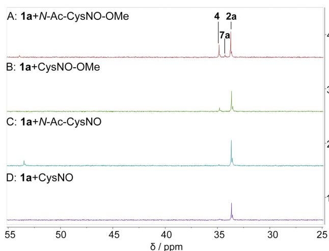
Figure 2. 31 P NMR for reaction of 1a (0.02 mmol) with CysNO and its derivatives (0.01 mmol): A) N -acetyl-CysNO-methyl ester, B) CysNO-methyl ester, C) N -acetyl-CysNO, D) CysNO in CD 3 CN/THF/Tris-HCl Buffer (100 mM, pH 7.4, 3:1:2) in dark after 30 min.
