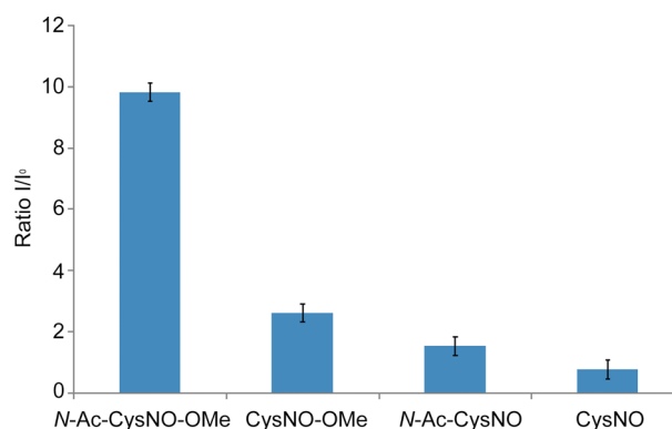
Figure 3. Fluorescence responses of 1b (40 \mu M) in CH 3 CN/PBS at rt for 60 min after addition of CysNO derivatives (2 equiv). Data are the average \pm SD of two independent experiments.
