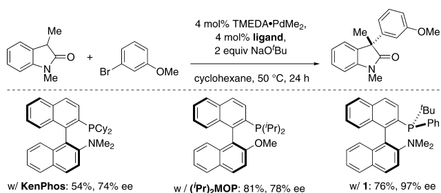
Figure 1. Pd-catalyzed enantioselective \alpha -arylation of 1,3-dimethyloxindole with an axially chiral, P-chirogenic ligand.
