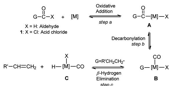
Scheme 1. Reaction of Aldehydes and Acid Chlorides with a Catalyst Center
