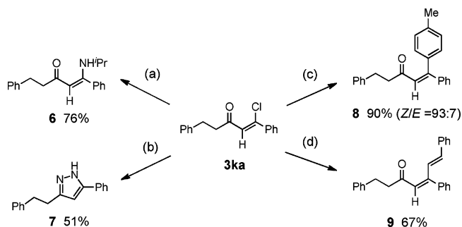
Scheme 2. Transformation of β-Chloroalkenyl Ketone 3ka a
