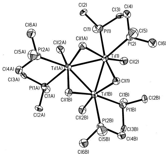
Fig. 7. Perspective drawing of the trinuclear [\text{Ti}(\mu\text{-Cl})\text{Cl}(\text{dmpe})]_3 cluster showing the atom labeling scheme. Atoms are represented by their thermal ellipsoids at 40% probability level. Hydrogen atoms are omitted for clarity.
