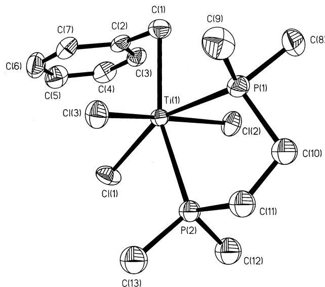
Fig. 2. Perspective drawing of the \text{TiCl}_3(\text{PhCH}_2)(\text{dmpe}) molecule showing the atom labeling scheme. Atoms are represented by their thermal ellipsoids at 40% probability level. Hydrogen atoms are omitted for clarity.
