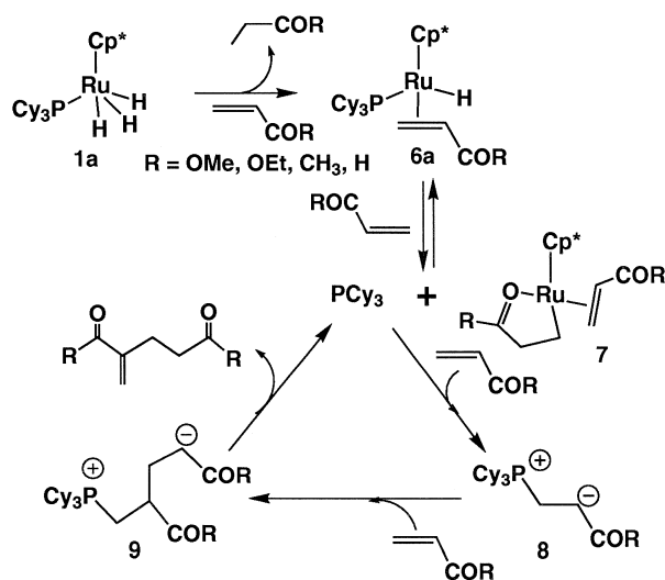
Scheme 1. A plausible mechanism of the ruthenium-mediated head-to-tail dimerization of acrylic compounds.
