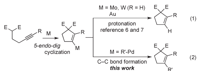
Scheme 1. Fate of Vinylmetal Intermediate Generated by 5- Endo-Dig Cyclization
