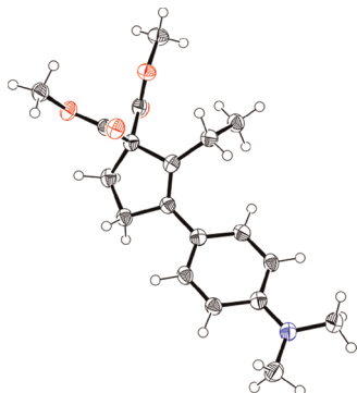
Figure 2. ORTEP drawing of compound 2af .
