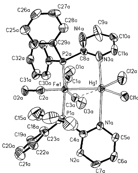
Fig. 2. Molecular structure and atom numbering of [(CO) 3 Fe(Ph 2 Ppym- N,N' ) 2 HgCl 2 ] 2 2a . The thermal ellipsoids are drawn at the 35% probability level.
