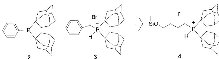
Scheme 3. Low molecular weight analogues 2–4 of the MeOPEG-tagged (1\text{-Ad})_2 -phosphines.
