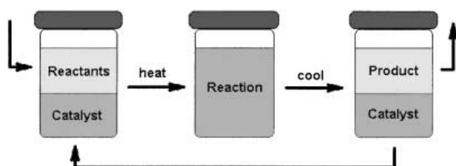
Figure 1. Biphasic catalysis.
