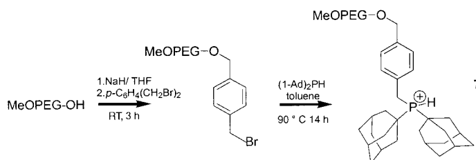
Scheme 6. Synthesis of 7 .
