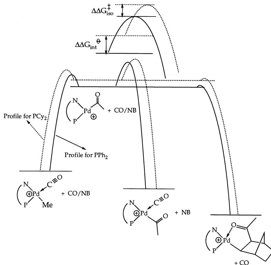
Fig. 3. Qualitative energy diagram for formation of (P,N)-Pd(COMe) + .
