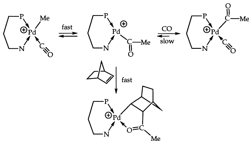
Scheme 1. Reaction pathways for the reaction of (P,N)\text{-PdMe(CO)}^+ with CO and norbornene.
