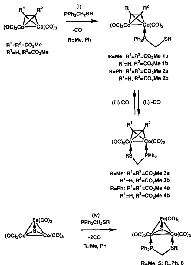
Scheme 1. Reagents and conditions for the formation of the new complexes. (i) PPh_2CH_2SR , toluene, 40°C; (ii) toluene, 60°C; (iii) CO, toluene, 60°C.
