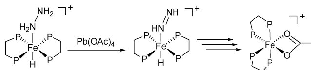
Scheme 4. Suggested Pathway for the Formation of \text{cis-}[\text{Fe}(\text{DMeOPrPE})_2(\text{O}_2\text{CCH}_3)]^+ from the Reaction of 9 with \text{Pb}(\text{OAc})_4
