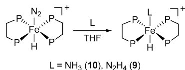
Scheme 2. Substitution of the \text{N}_2 Ligand on 7 with Ammonia or Hydrazine Leading to 10 or 9 , Respectively
