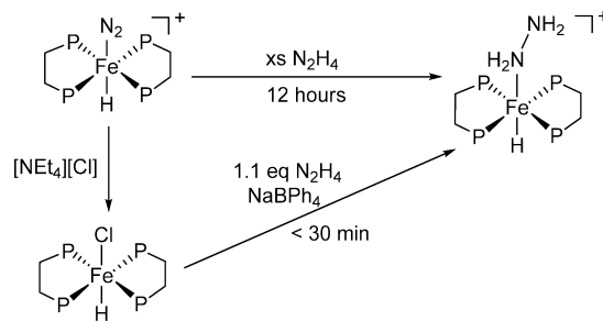
Scheme 3. Synthesis of 9 by Substitution of the N 2 Ligand of 7 (Top) or by Abstraction of the Cl Ligand from trans -Fe(DMeOPrPE) 2 (Cl)H (Bottom)
