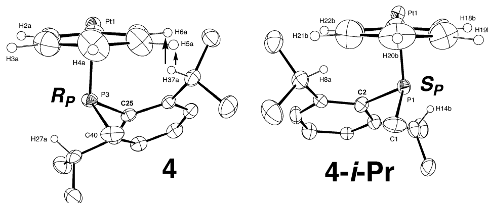
Figure 4. Partial ORTEP diagrams ( p - i -Pr groups omitted) for the complexes ( R_P )-Pt(( R,R )-Me-Duphos)(Ph)(PMeIs) ( 4 ) and ( S_P )-Pt(( R,R )- i -Pr-Duphos)(Ph)(PMeIs) ( 4- i -Pr , one of the two independent molecules in the unit cell), illustrating close contacts between ortho i -Pr CH groups H37 (in 4 ) and H8 (in 4- i -Pr ) and the Pt–Ph ring. The arrows on the left show NOEs observed between i -Pr CH H37 and Pt–Ph hydrogens H5 and H6.
