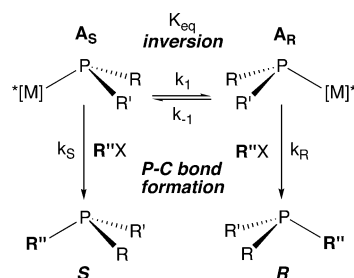
Scheme 1. Phosphorus Inversion and Alkylation in Diastereomeric Metal Phosphido Complexes a
