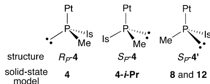
Chart 1. Possible Phosphido Configurations in the Major Diastereomer of 4 , with Solid-State Models
