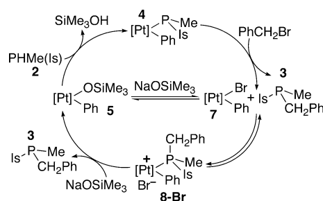
Scheme 10 a
