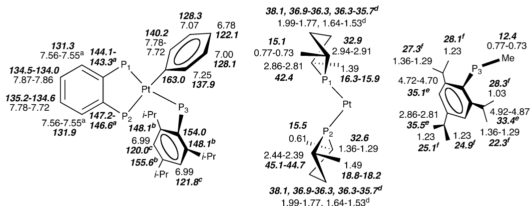
Chart 2. ^1\text{H} and ^{13}\text{C} (Boldface Italics) NMR Assignments for the Major Diastereomer of 4 ( \text{THF-d}_8 , -60^\circ\text{C} )
