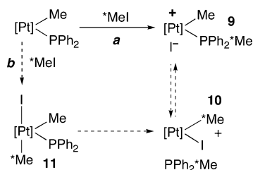
Scheme 7 a
