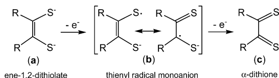
Scheme 2. Possible Oxidation States of a Dithiolene Ligand
