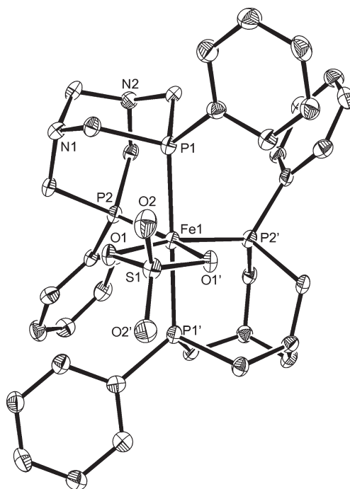
Figure 1. Molecular structure of [Fe(κ 2 -O 2 SO 2 )L 2 ] ( 1 ), from the crystal structure of 1 ·2H 2 O. Ellipsoids are represented at 30% probability. Hydrogen atoms have been omitted for clarity. Primed labels are related to those in the asymmetric unit by the -x, y, -z + \frac{1}{2} symmetry operation.
