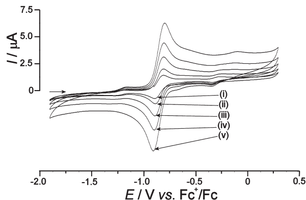
Figure 7. Cyclic voltammograms for the oxidation of 1 mM trans - [\text{FeCl(H)L}_2] ( 7 ) at a 1 mm diameter Pt electrode in 1,2-dichloroethane/0.1 M \text{NBu}_4\text{PF}_6 at scan rates of (i) 10 \text{ mV s}^{-1} , (ii) 20 \text{ mV s}^{-1} , (iii) 50 \text{ mV s}^{-1} , (iv) 100 \text{ mV s}^{-1} , and (v) 200 \text{ mV s}^{-1} .
