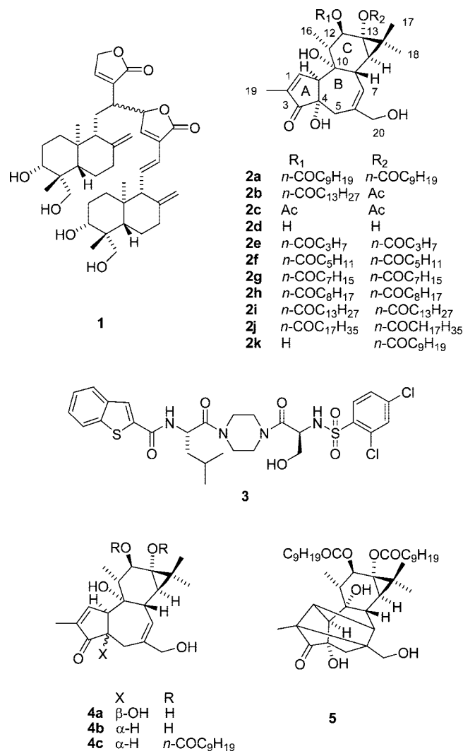
Figure 1. Structural formulas of the TRPV4 ligands BAA ( 1 ), 4α-PDD ( 2a ), GSK1016790A ( 3 ), of the new ligands investigated ( 2e–k , 4a–c , and 5 ), and of the reference phorboids 2b–d .
