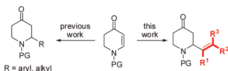
Scheme 1. Reported and This Work on the ACA to 2,3-Dihydro-4-piperidones
