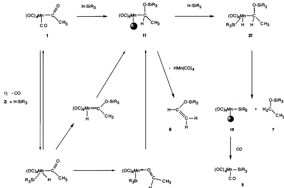
Scheme 7. Intramolecular Pathways for \text{HSiR}_3 and (\text{CO})_5\text{MnC}(\text{O})\text{CH}_3 ( 1 )
