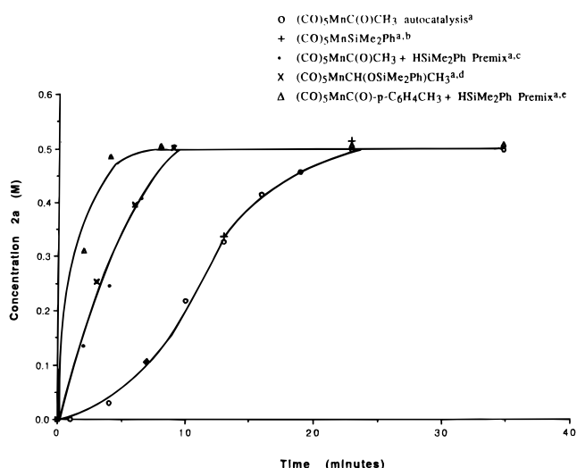
Figure 4. Reaction profiles: dimethyphenylsilane autocatalyzed hydrosilylation of (\text{CO})_5\text{Mn}(\text{C}(\text{O})\text{CH}_3) ( 1 ). Conditions: (a) (\text{CO})_5\text{Mn}(\text{C}(\text{O})\text{CH}_3) ( 1 ) (100 mg, 0.42 mmol), \text{Me}_2\text{PhSiH} (65 mg, 0.48 mmol, 1.1 equiv), and anisole (60 mg, 0.55 mmol) in 600 mg of \text{C}_6\text{D}_6 (25 °C). All concentrations were determined by quantitative ^1\text{H} NMR spectroscopy (vs anisole). (b) (\text{CO})_5\text{MnSiMe}_2\text{Ph} ( 5a ) (2 mg, 0.0063 mmol, 1.5%) added. (c) Catalyst premix: (\text{CO})_5\text{Mn}(\text{C}(\text{O})\text{CH}_3) ( 1 ) (3 mg, 0.008 mmol, 1.9%) and \text{Me}_2\text{PhSiH} (65 mg, 0.48 mmol) in 600 mg of \text{C}_6\text{D}_6 reacted 45 min prior to addition of 1 (100 mg, 0.42 mmol). (d) (\text{CO})_5\text{MnCH}(\text{OSiMe}_2\text{Ph})\text{CH}_3 ( 2a ) (3 mg, 0.008 mmol, 1.9%) added. (e) Catalyst premix: (\text{CO})_5\text{Mn}(\text{C}(\text{O})-p\text{-C}_6\text{H}_4\text{CH}_3) (1 mg, 0.003 mmol, 0.9%) and \text{HSiMe}_2\text{Ph} (65 mg, 0.48 mmol) in 600 mg of \text{C}_6\text{D}_6 reacted 45 min prior to addition of 1 (100 mg, 0.42 mmol).
