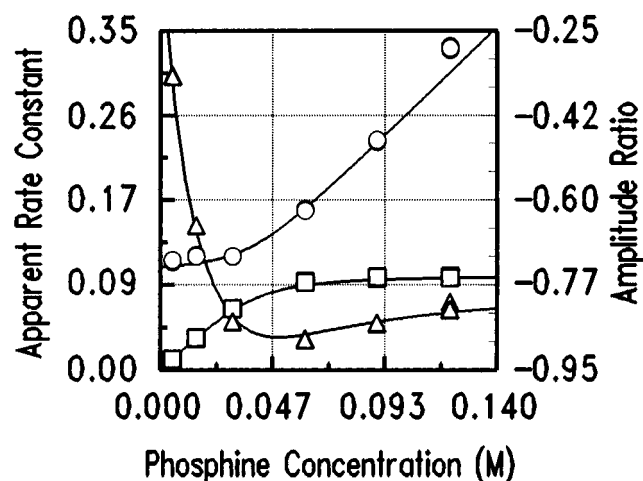
Figure 4. Dependence of the biexponential fit parameters on concentration of phosphine for the reaction of 1a with \text{P}(p\text{-PhOMe})_3 at 30 °C. The lower rate constant, \lambda_1 (□), and the higher rate constant, \lambda_2 (○), are plotted against the left abscissa, and the amplitude ratio, A_1/A_2 (Δ), is plotted against the right abscissa. Each parameter at each concentration is presented in triplicate. The solid lines are calculated from the fit to all of the data, using the parameters in Table 2.
