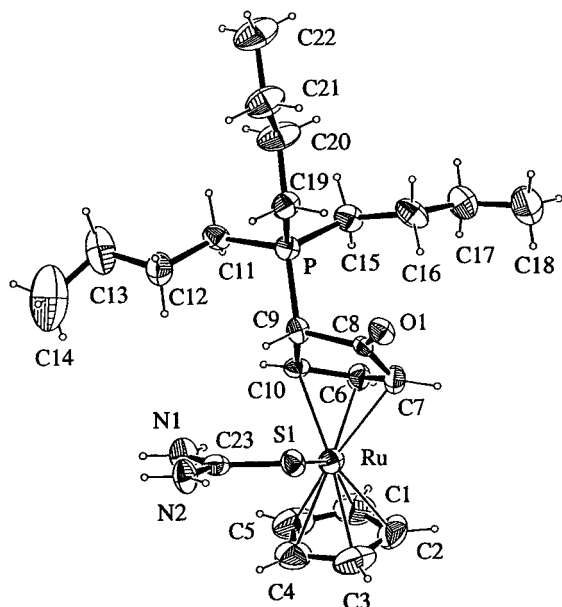
Figure 2. Structural view of [\text{Ru}(\eta^5\text{-C}_5\text{H}_5)(\eta^3\text{-C}_5\text{H}_4\text{O-2-PBu}^u_3)(\text{tu})](\text{CF}_3\text{SO}_3) ( 10a ). Selected bond lengths (Å) and angles (deg) are as follows: Ru–S(1), 2.394(4); Ru–C(7), 2.226(11); Ru–C(6), 2.054(11); Ru–C(10), 2.181(10); Ru–C(1–5) av , 2.199(10); C(8)–O(1), 1.219(13); C(9)–P, 1.810(5); S(1)–C(23), 1.694(13); C(23)–N(1), 1.333(9); C(7)–C(6)–C(10), 106.6(10); Ru–S(1)–C(23), 110.2(3); C(7)–C(8)–C(9), 105.4(10).
