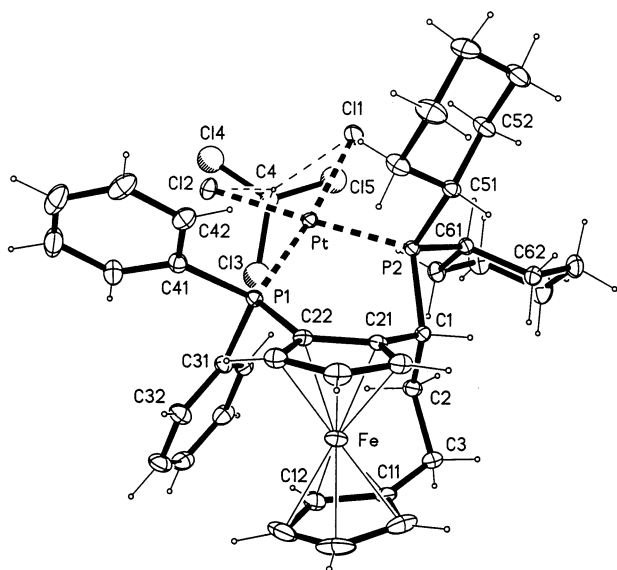
Fig. 2. Structural view of 2a ·CHCl 3 showing 20% probability thermal ellipsoids. The CHCl 3 solvent molecule behind the PtP 2 Cl 2 quadrangle and its bifurcated hydrogen bond to Cl1 and Cl2 (thin dashed line) is included.
