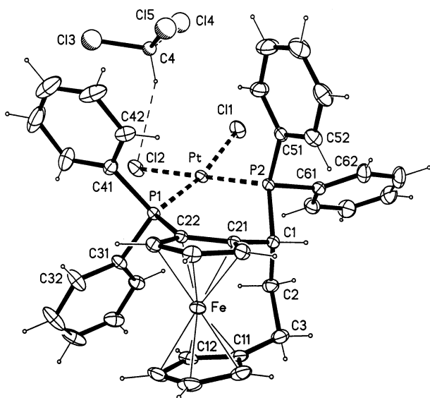
Fig. 1. Structural view of 1a ·CHCl 3 showing 20% probability thermal ellipsoids. The CHCl 3 solvent molecule and its hydrogen bond to Cl2 (thin dashed line) is included.
