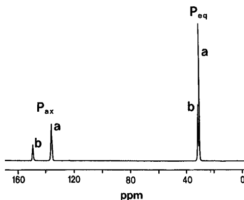
Figure 2. ^{31}\text{P} NMR spectra of the chloro (a) and iodo (b) complexes in the equilibrium in deuterated chloroform.
