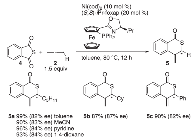
Scheme 4. Nickel-Catalyzed Asymmetric Decarbonylative Cycloaddition of Thiophthalic Anhydride 4 with Allene 2
